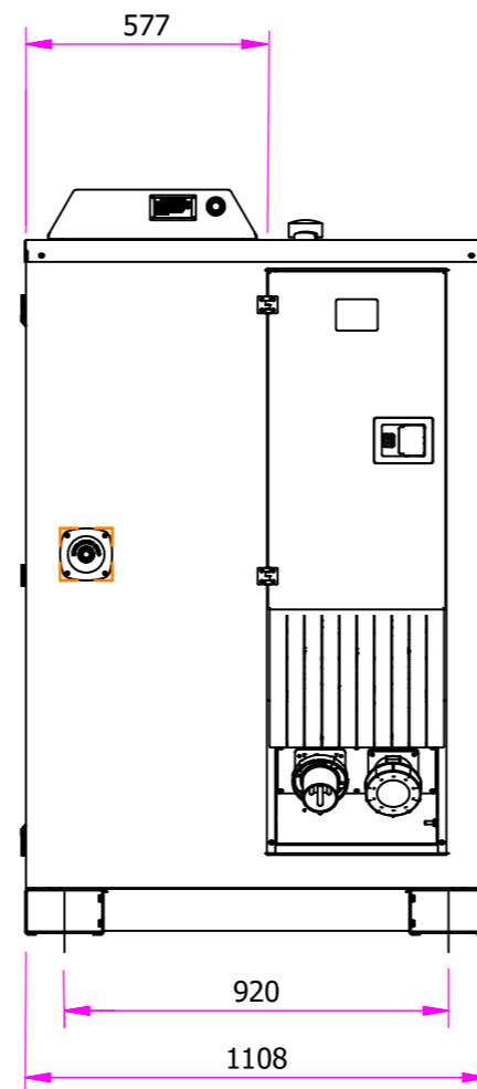
P473-01-01 GA - EASYGRID 45000 GA SCALE: (1:20)
